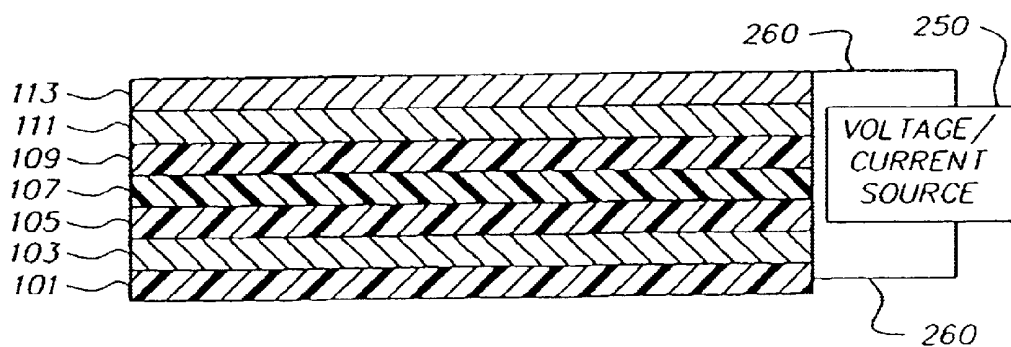
FIG. 3 (PRIOR ART)
